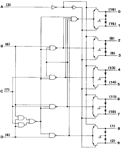
logic diagram
